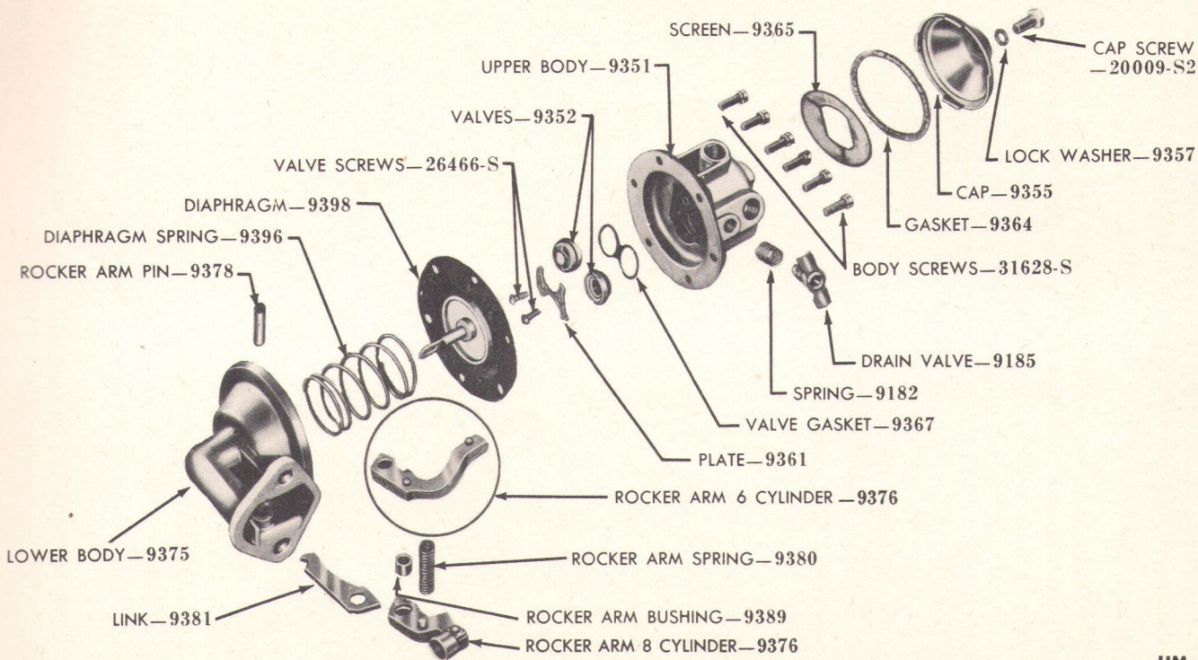
Figure 22—Fuel Pump Disassembled (6, 8, and 12-Cylinder)
